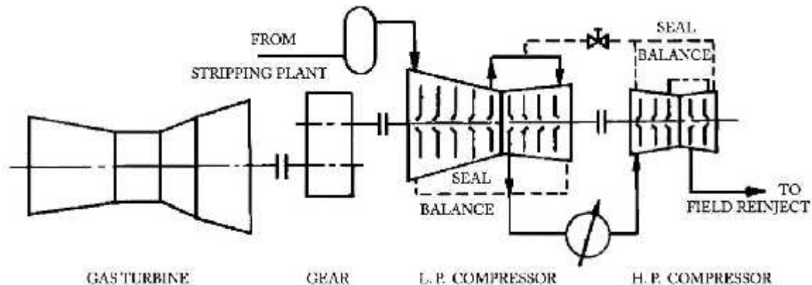
Figure 1: Kaybob Compressor Train Schematic. From Smith [3].
