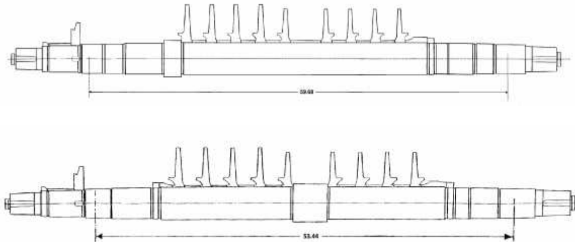
Figure 4: Rotor redesign. From Smith [3].
