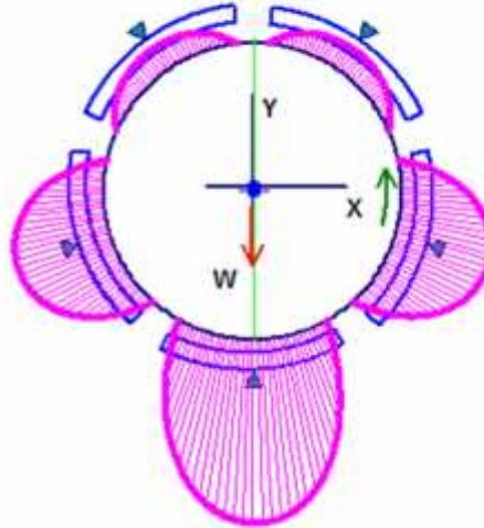
Figure 11: Original Compressor Bearing Analysis Results.
