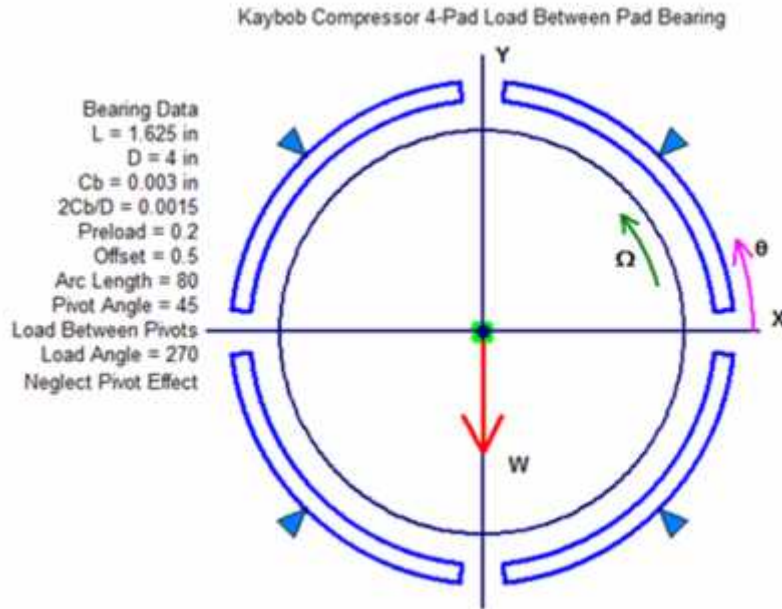
Figure 17: Initial Four Pad Bearing Design.
