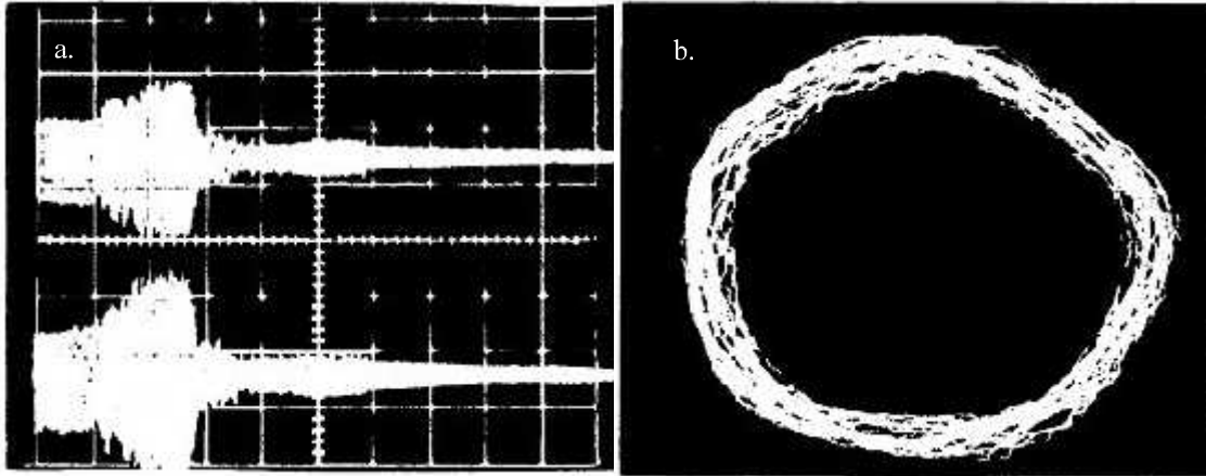
Figure 2: (a) Time-lapse and (b) orbit of the instability onset. From Smith [3].
