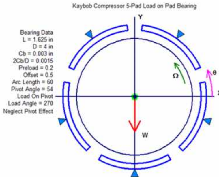
Figure 10: Original Compressor Bearing Design.
