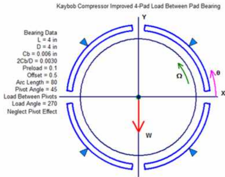
Figure 20: Improved Four Pad Bearing Design.
