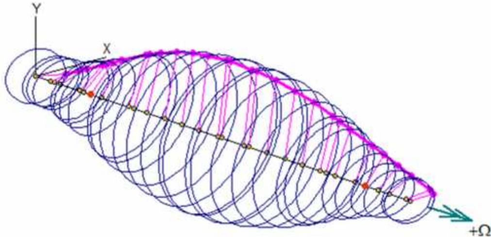
Figure 30: Stability Analysis of the New Rotor Design with the Original Bearing and a Long Squeeze Film Damper.
