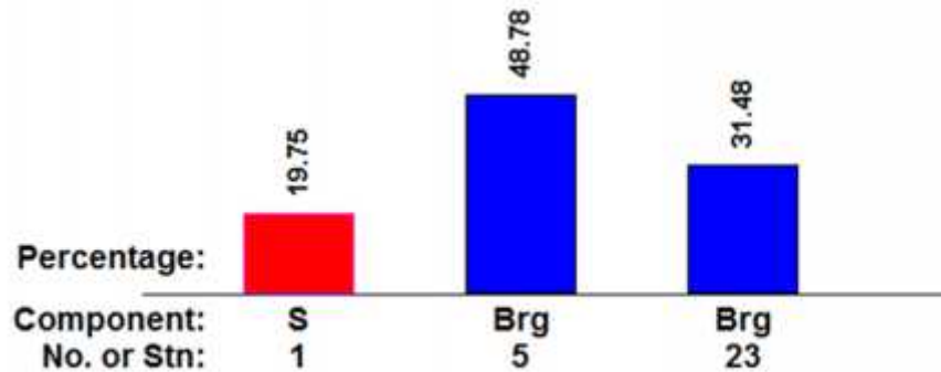
Figure 23: Energy Distribution in the Shaft and Bearings for the Improved Four Pad Bearing Design.
