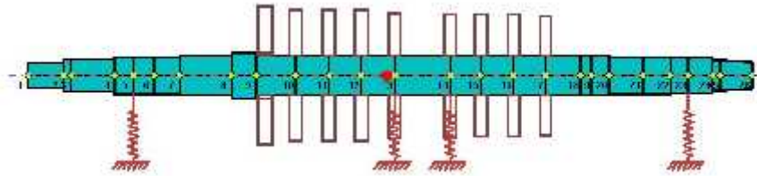
Figure 5: Kaybob 9 Stage Compressor Model with Aerodynamic Cross Coupling at Stations 13 and 14.
