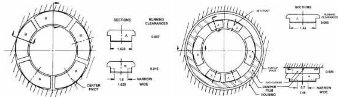
Figure 3: (a) Asymmetric Tilt Pad Bearing and (b) Squeeze Film Damper Design. From Smith [3].
