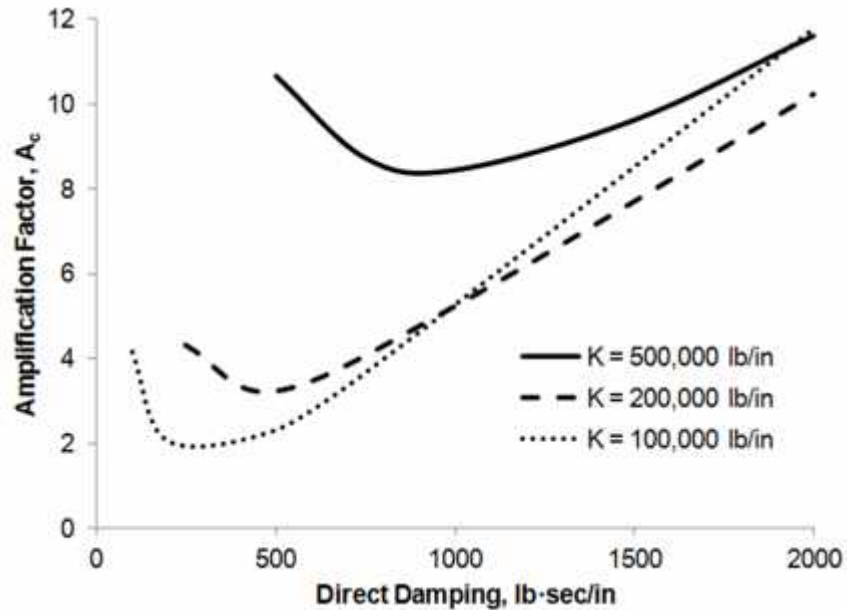
Figure 9: Amplification Factors of the First Bending Mode.
