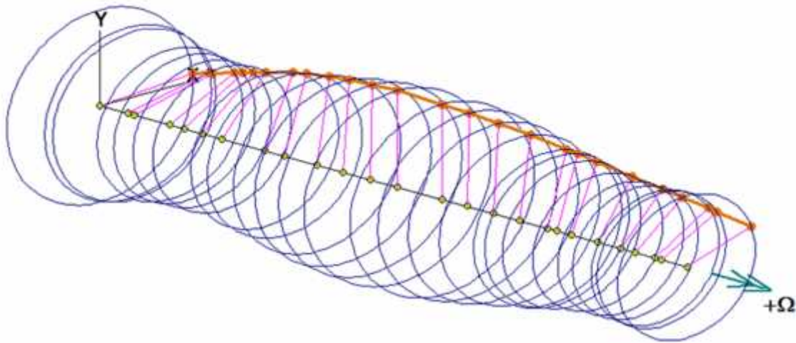
Figure 22: Stability Analysis of the Improved Four Pad Bearing.
