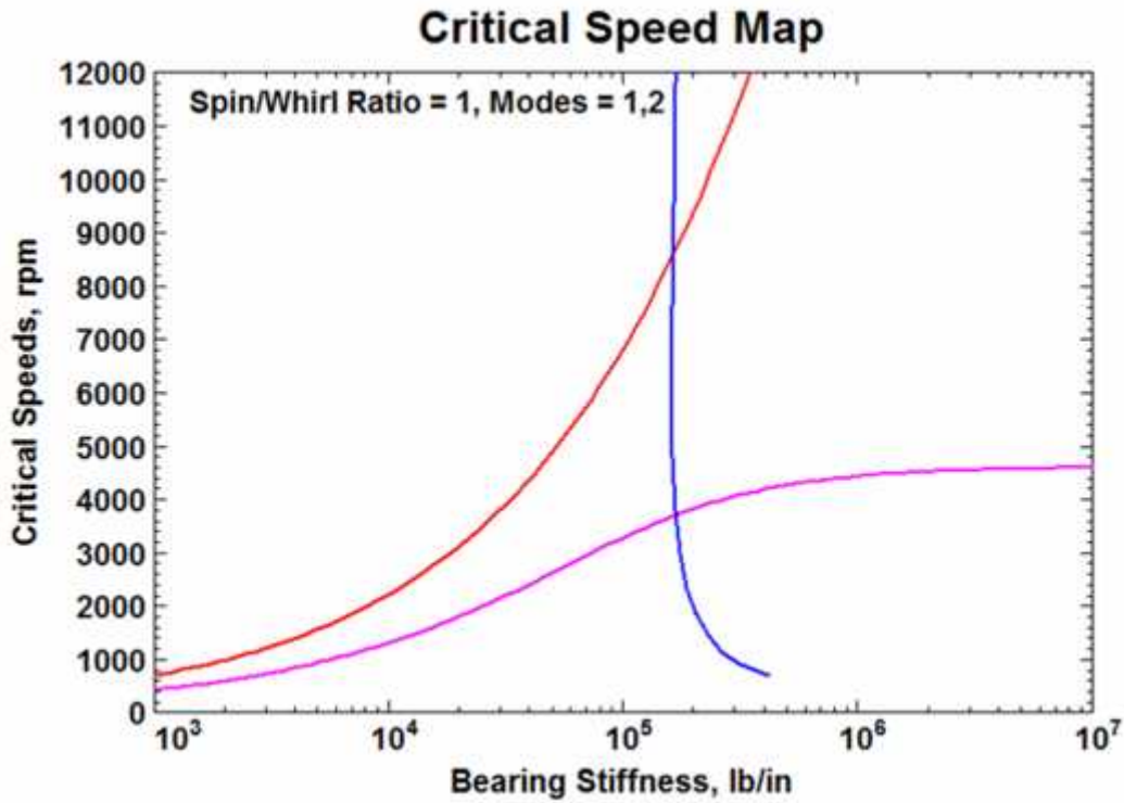
Figure 6: Compressor Critical Speed Map.
