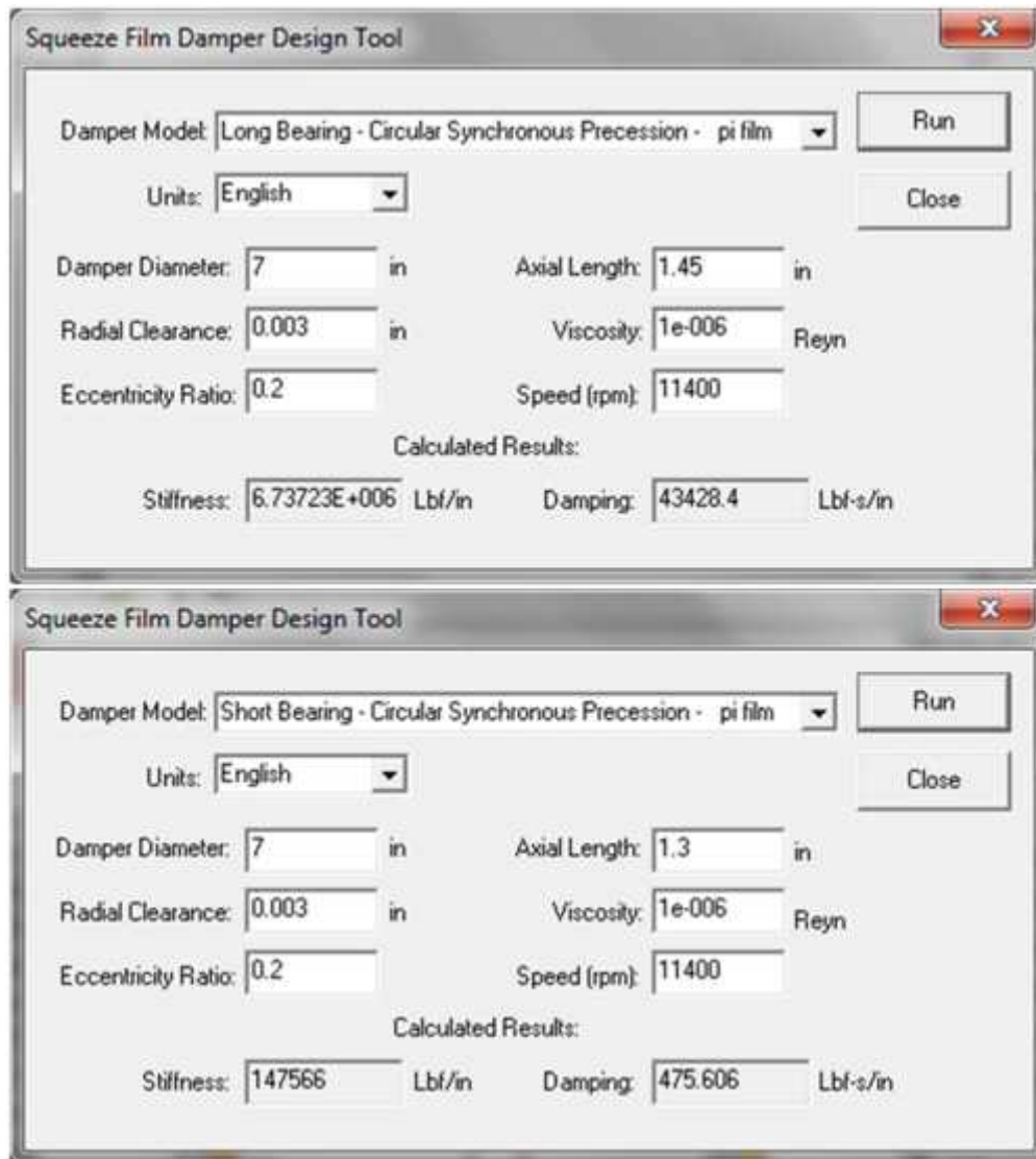
Figure 24: Non-Grooved and Grooved Squeeze Film Damper Analysis.
