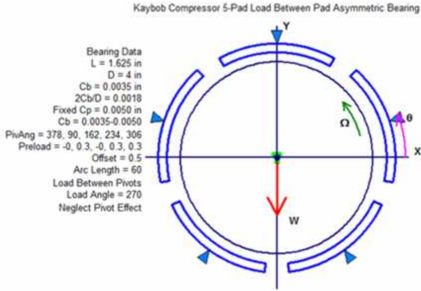
Figure 14: Asymmetric Bearing Model.
