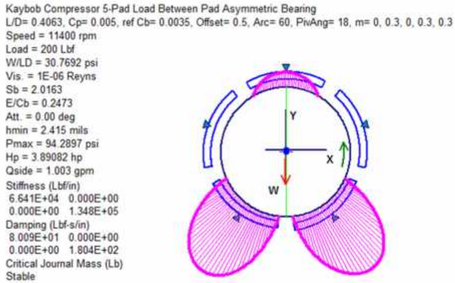
Figure 14: Asymmetric Bearing Model.
