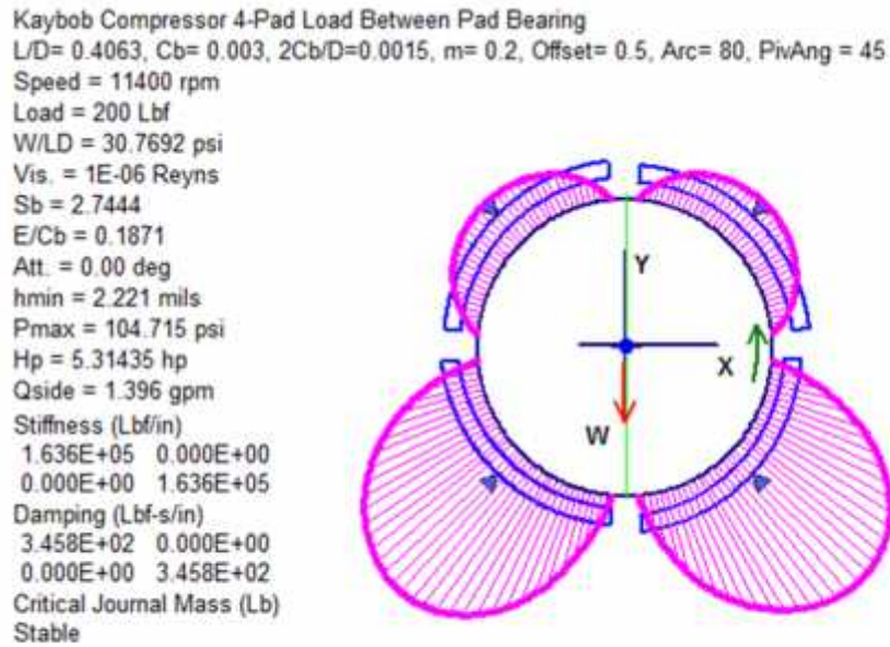
Figure 17: Initial Four Pad Bearing Design.
